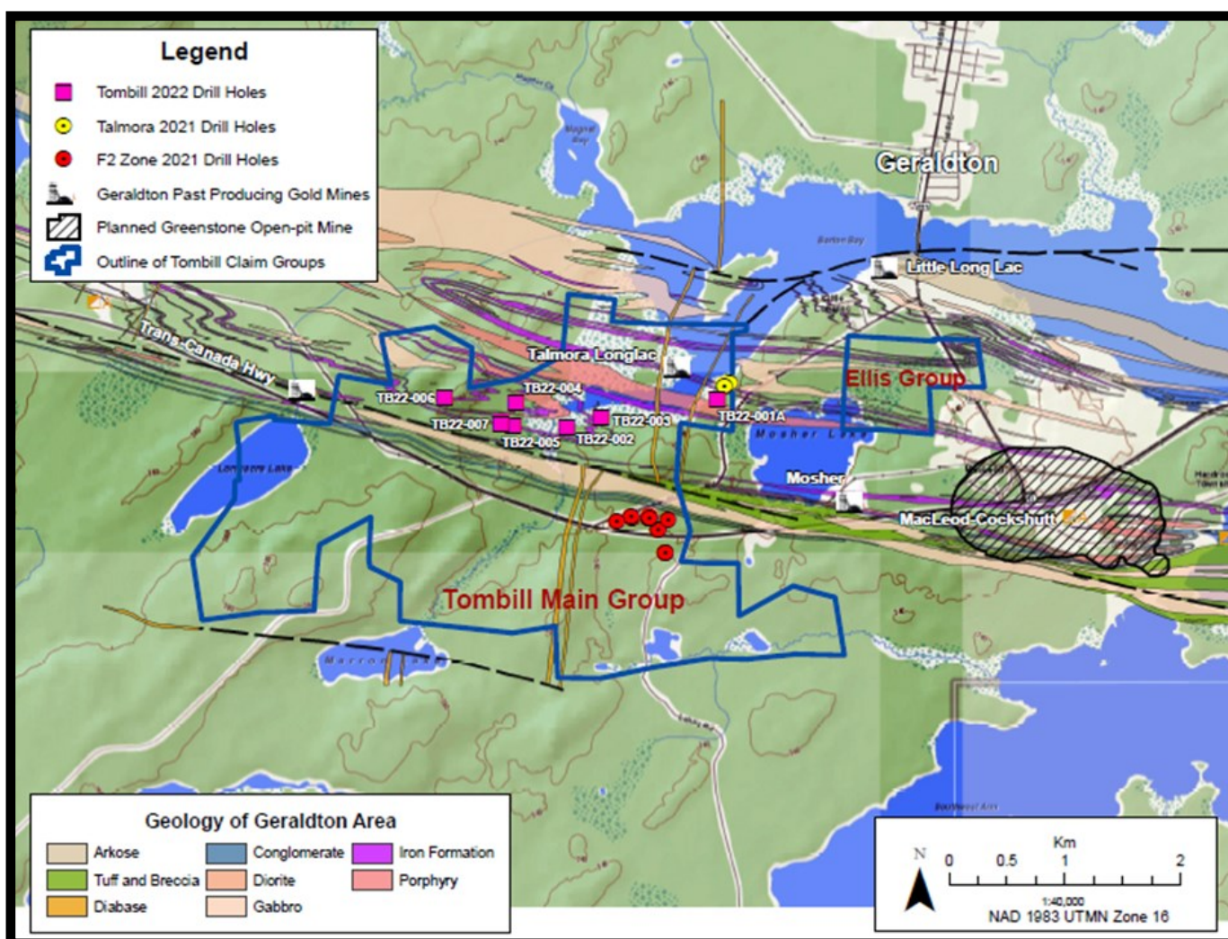
Figure 1. Regional map showing location of Tombill mineral properties in the Geraldton gold mining district and collar locations of diamond drill-holes completed by the Company's 2021 and 2022 drilling campaigns.
